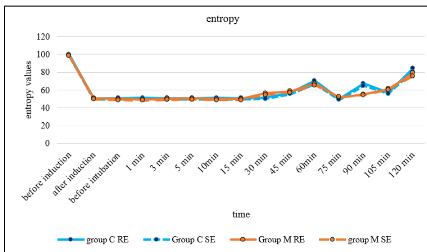
Fig. 2: Comparison of entropy between group C and group M
